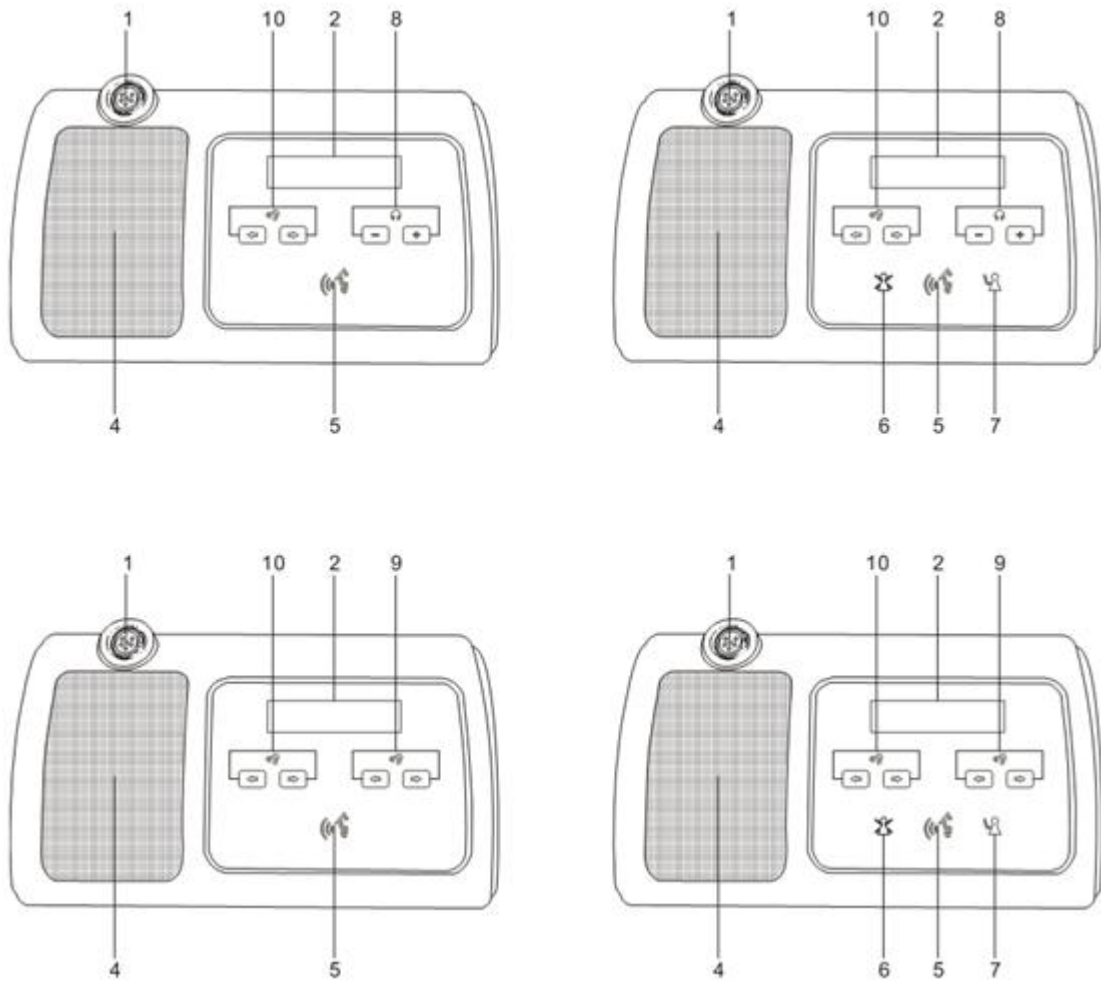
Figure 3.1.1.2 Top view of wired units DCS-DIC/DID/DSC/DSD-T
