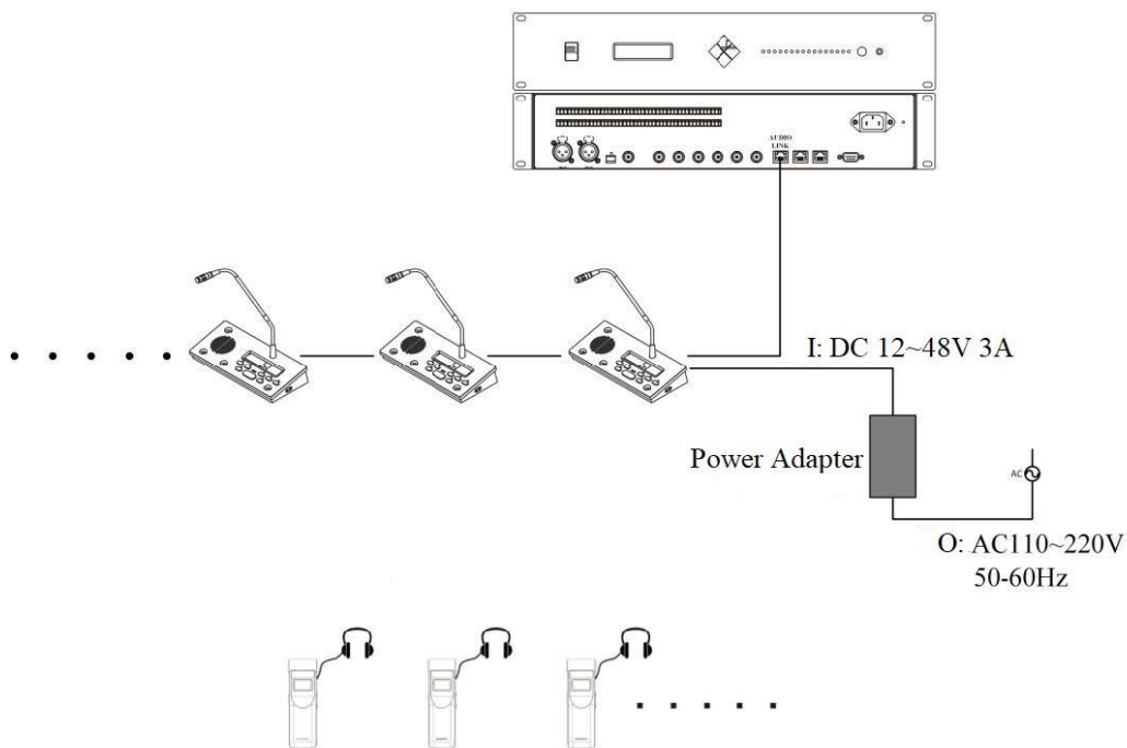
Figure 4.2.2 DCS-INT64 directly connected to infrared transmitter
