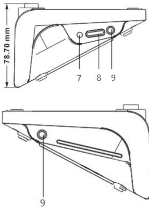
Figure 3.7.1.2 Left view and right view of DCS-MAW-T
