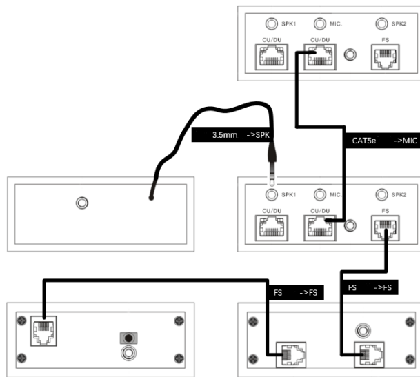
Figure 3.5.3 Connection of DCS-DCC/DCD/CSU/DVU/SPK-F/FS/FS1/FS2
