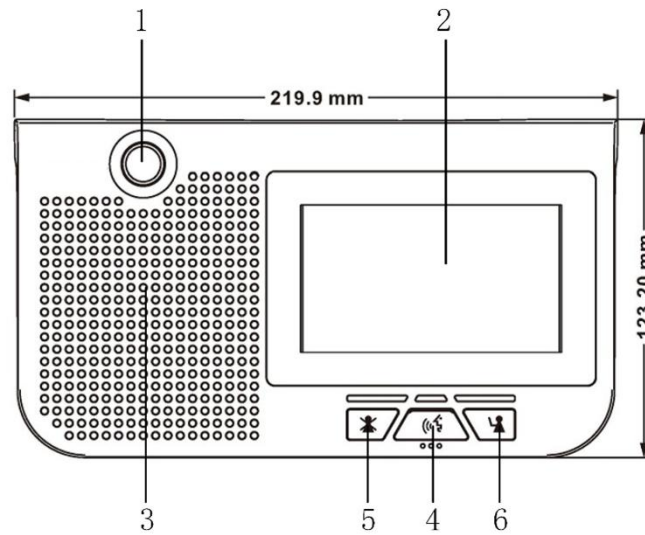
Figure 3.3.1.1 Top view of DCS-MAU-T
