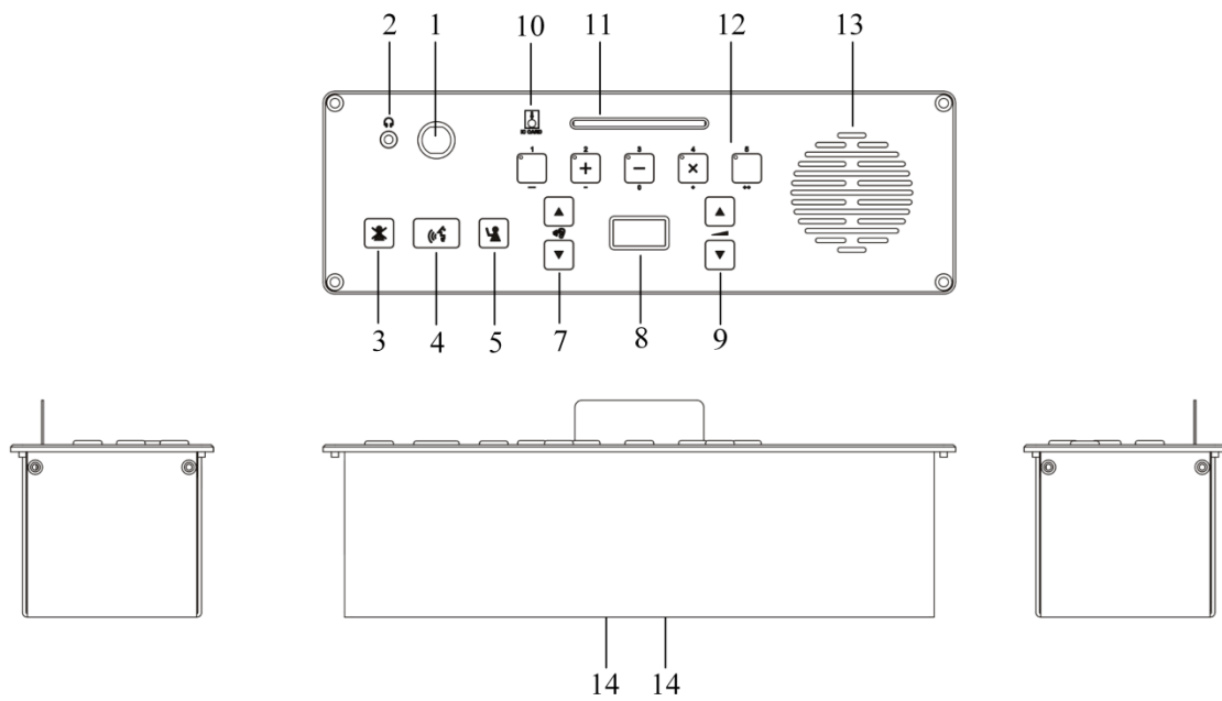
图 3.5.1.3 DCS-FFC/FFD-F1/F2 flush-mounting unit
