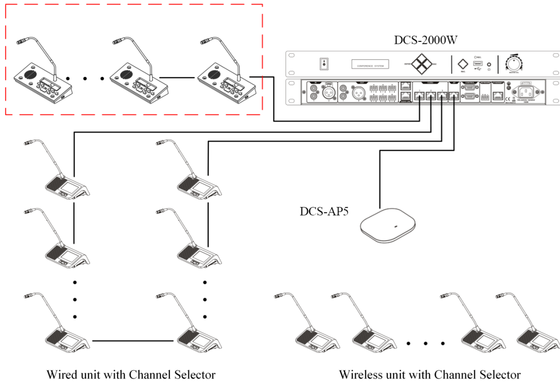
Figure 4.2.1 DCS-INT64 connected to controller
