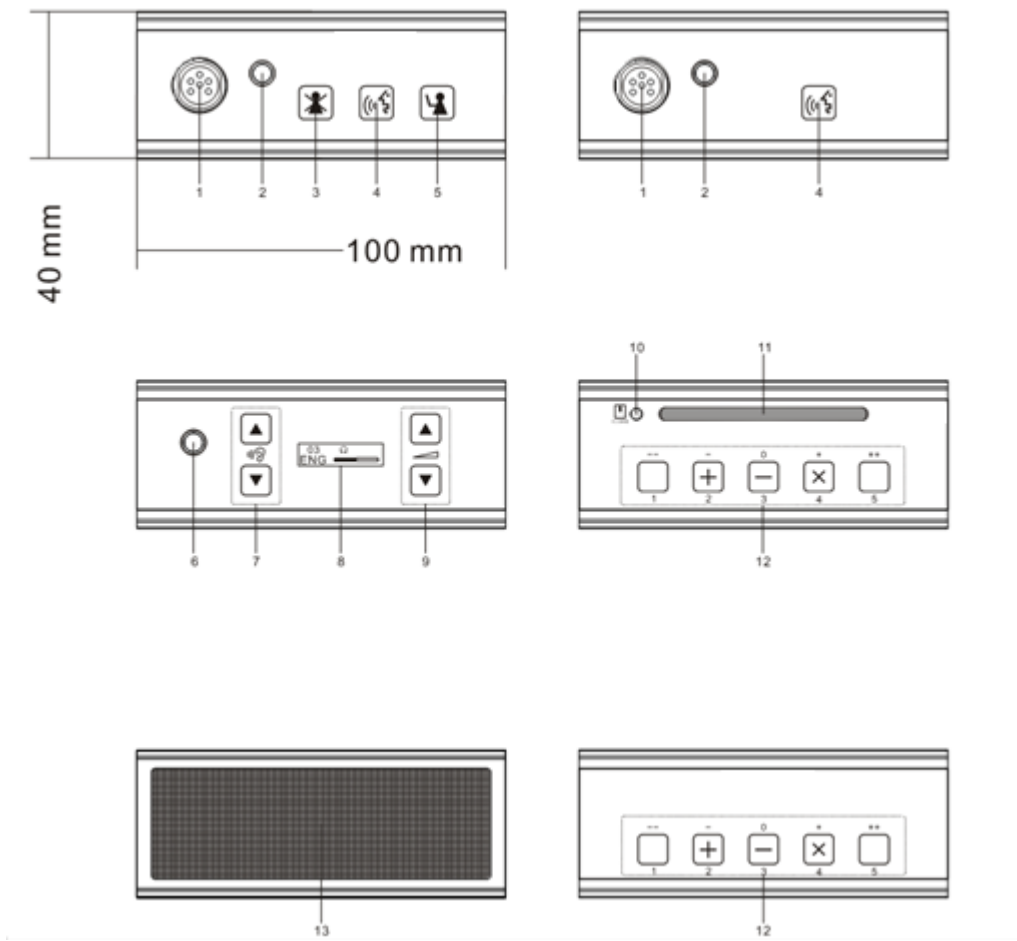
Figure 3.5.1.1 Front view of DCS-DCC/DCD/CSU/DVU/SPK-F/FS/FS1/FS2
