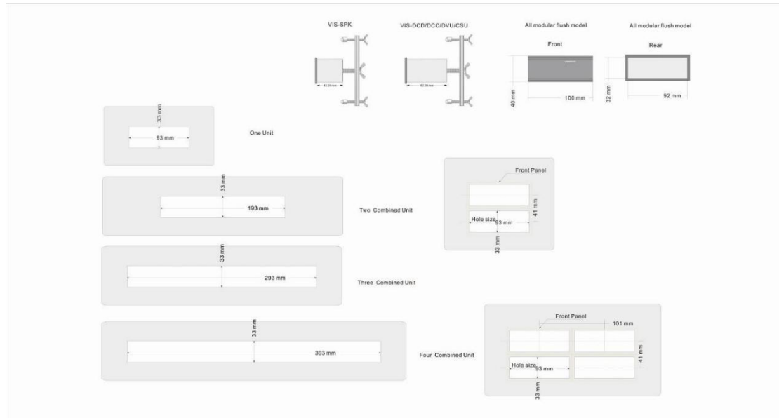
Figure 3.5.2.1.1 Sizes of mounting holes for DCS-DCC/DCC/DVU/SPK-F/FS/FS1/FS2
