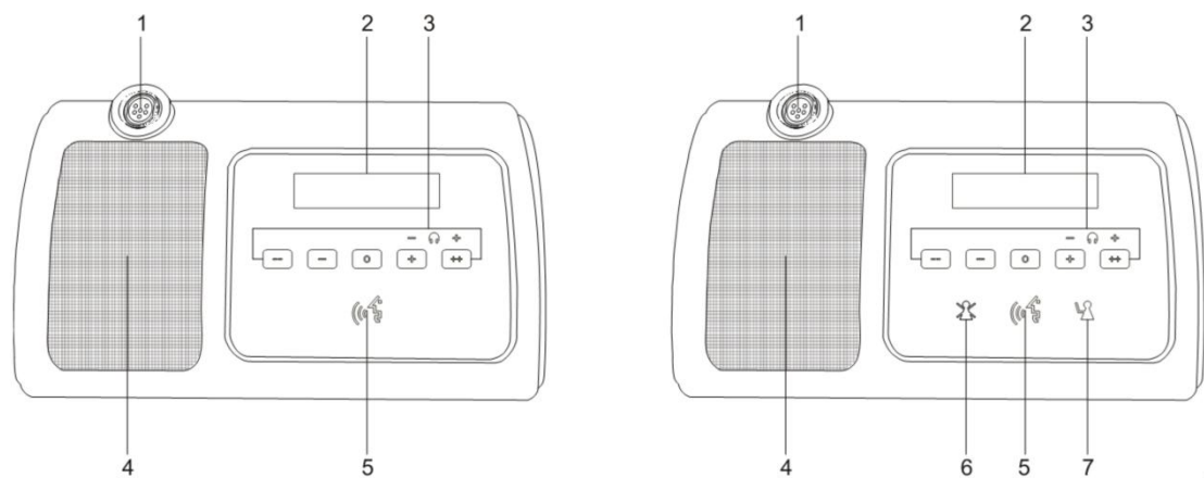
Figure 3.6.1.2 Top view of DCS-WVC/WVD/WVCIC/WVDIC-T
