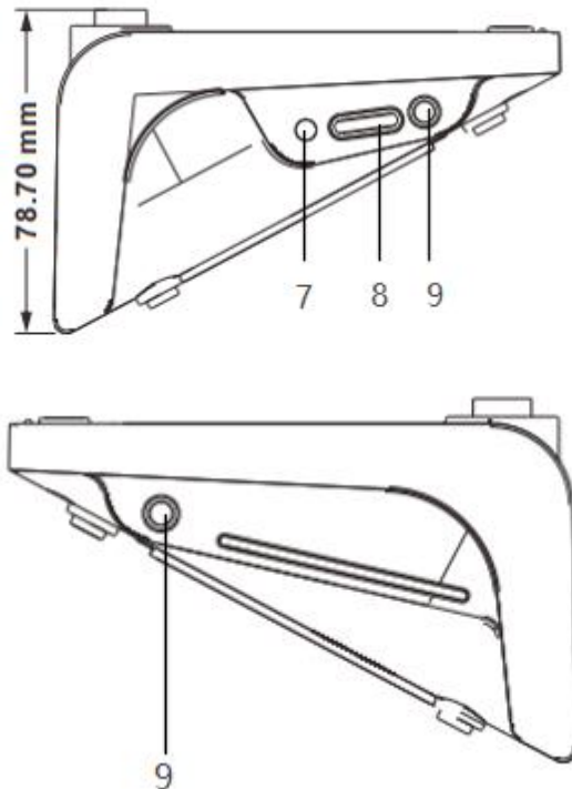
Figure 3.3.1.2 Left view and right view of DCS-MAU-T
