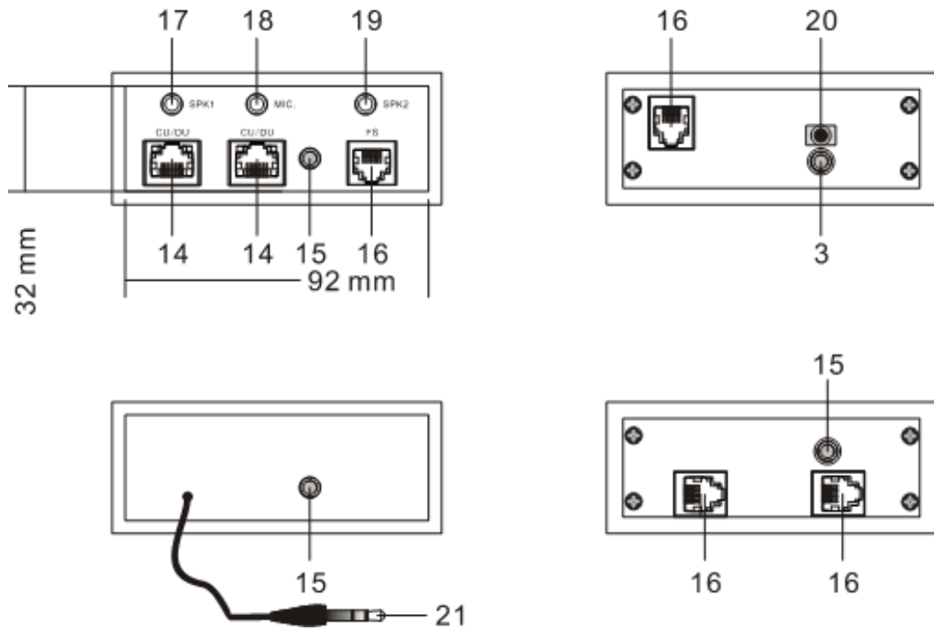
Figure 3.5.1.2 Rear view of DCS-DCC/DCD/CSU/DVU/SPK-F/FS/FS1/FS2
