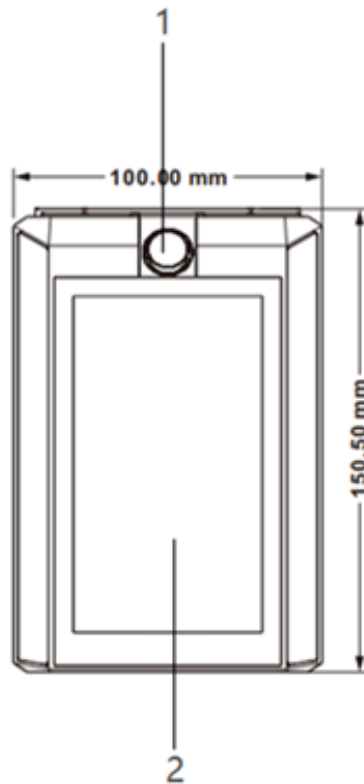
Figure 3.2.1.1 Top view of DCS-DMD-T
