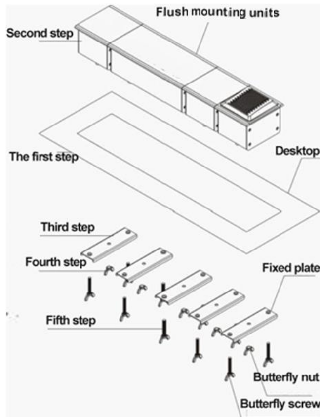
Figure 3.5.2.2 Installation steps of DCS-DCC/DCD/CSU/DVU/SPK-F/FS/FS1/FS2
