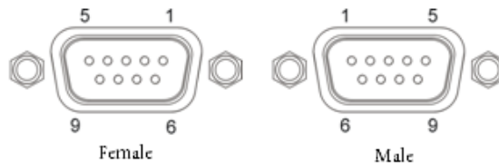
Figure 2.1.3.7.2 Pin descriptions of the CONTROL interface
